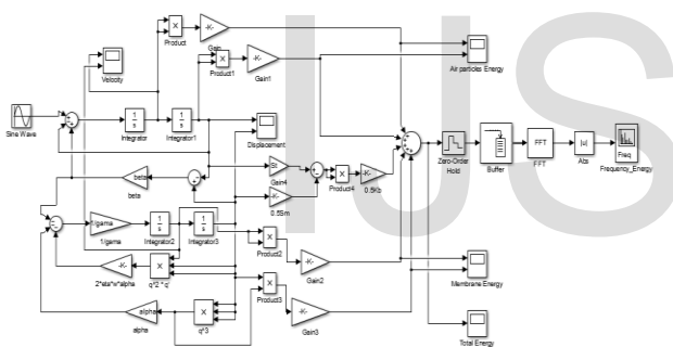
Figure 5.1: Simulink model based on equation of motion correspond to third boundary condition
