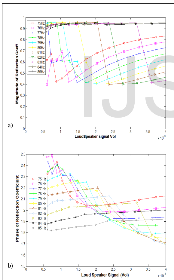
Figure 5. effect of NET in BC1 on tereflection coefficient. a) Magnitude; b) Phase.
