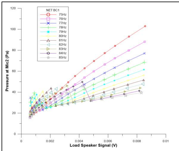
Figure 4. Pressure amplitude at the midsection of the duct (Mic.2) showing the occurrence of NET (BC1).
