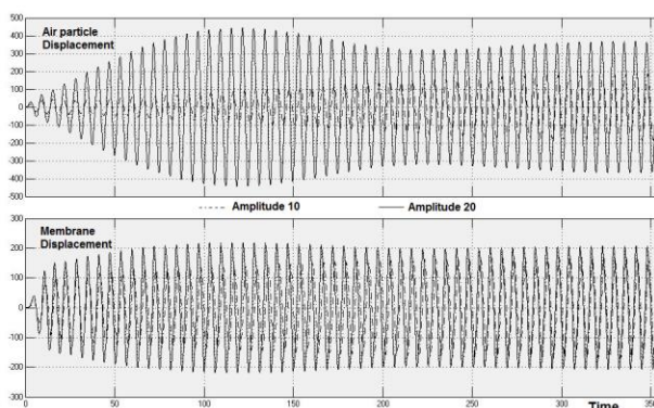
Figure 5.2: Numerical results of NET occurrence with two different amplitude applied to primary system
