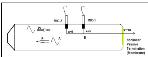
Figure 1. Schematic view of left and right moving waves in the plane wave region.
