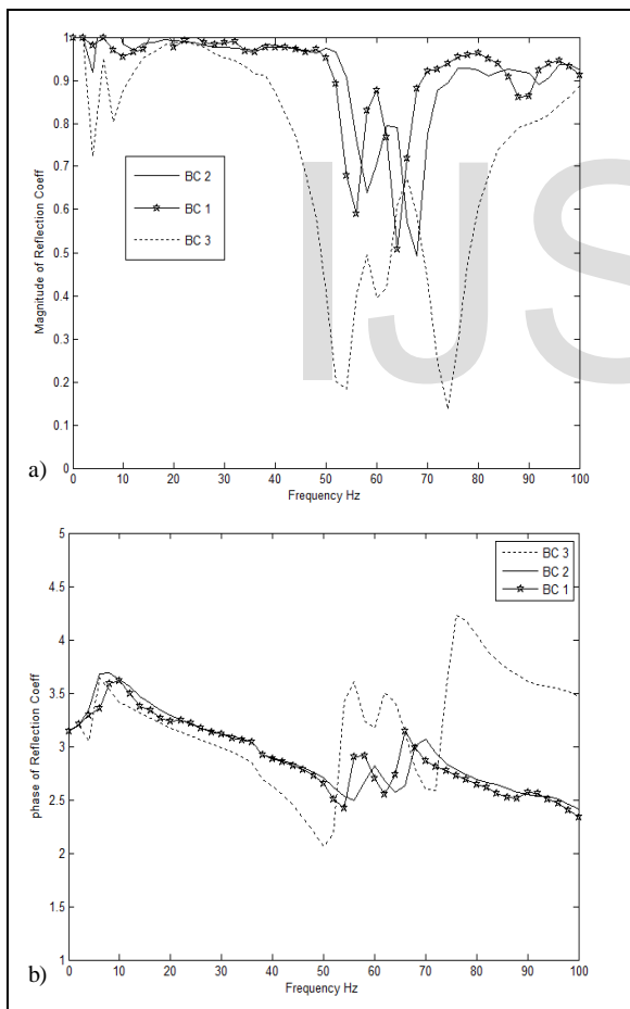
Figure 3. Reflection coefficient measured for 3 BCs at the end section of the duct under white noise excitation with low-level amplitude. a) Magnitude; b) Phase.
