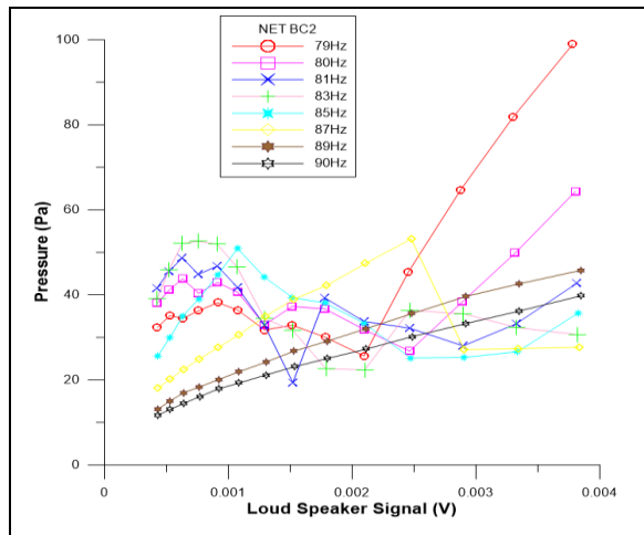
Figure 6. Pressure amplitude at the midsection of the duct (Mic.2) showing the occurrence of NET (BC2).
