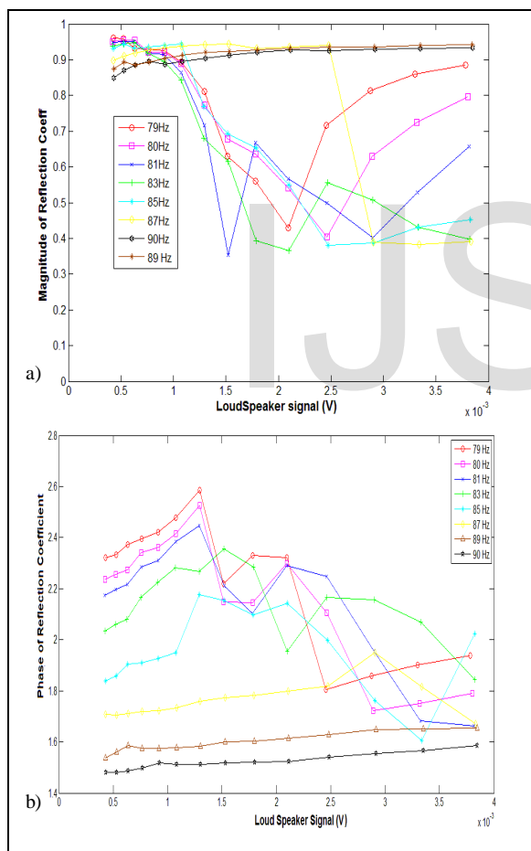
Figure 7. Effect of NET in BC2 on reflection coefficient. a) Magnitude; b) Phase.
