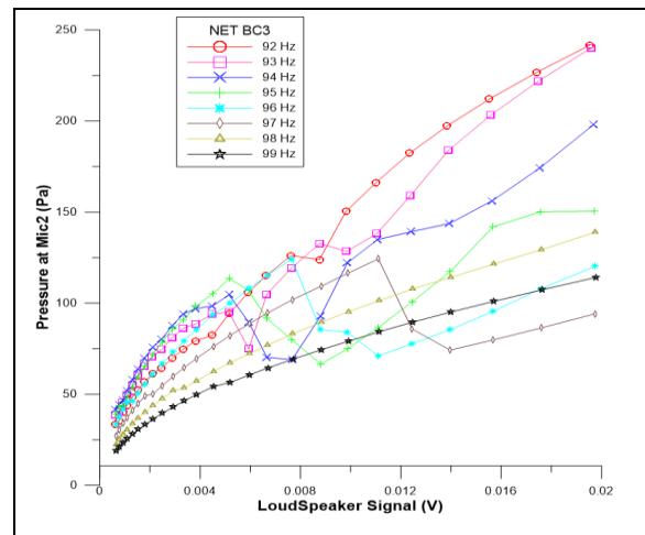
Figure 8. Pressure amplitude at the midsection of the duct (Mic.2) showing the occurrence of NET (BC3).
