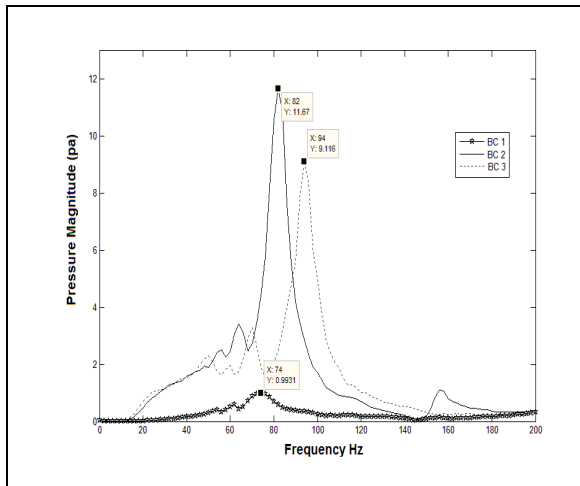
Figure 2. Pressure magnitude measured for 3 BCs by the microphone located in the middle section of the duct, under white noise excitation with low-level amplitude.
